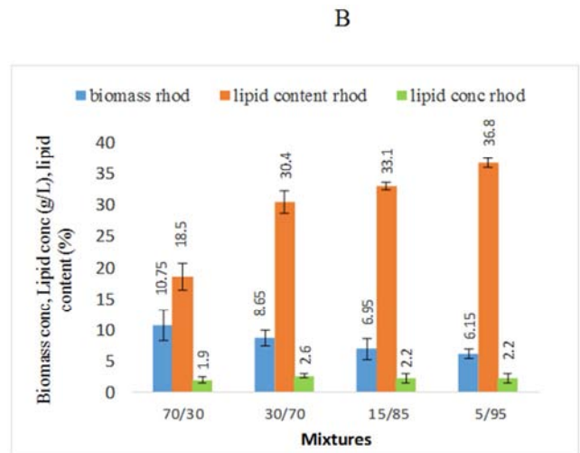
Figure 2. Biomass concentration, lipid concentration and lipid content comparison between different vinasse/glycerol mixture compositions. A: C. tropicalis , B: R. mucilaginosa .
