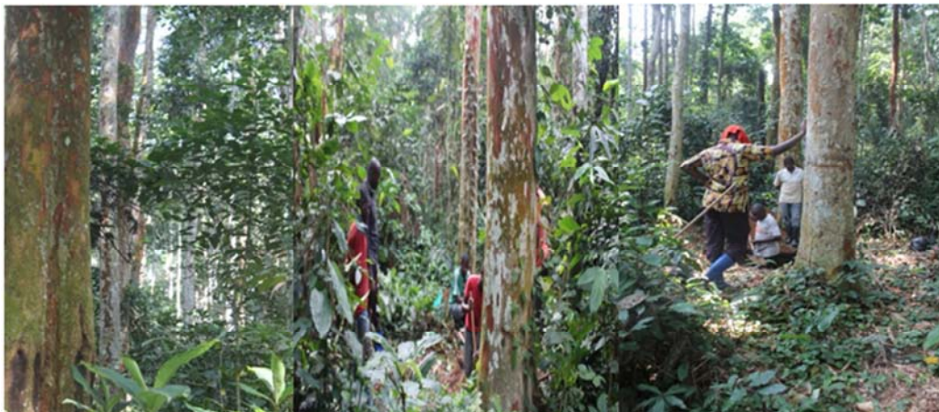
Figure 3. Pericopsis elata experimental plantations in Blanc-Etoc technique since 1938 in Yangambi, RD Congo (Photo taken in 2018)
