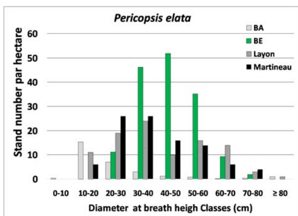
Figure 4. Individuals distribution of 82 year old Pericopsis elata per diameter class under four silvicultural techniques in Yangambi, DR Congo.
