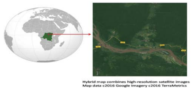
Figure 1. Yangambi evergreen dense humid forest reserve crossed by the Congo river (to the right) located to the Northern DR Congo in red pointed on the world map (to the left) (Source: Google map, 2016).
