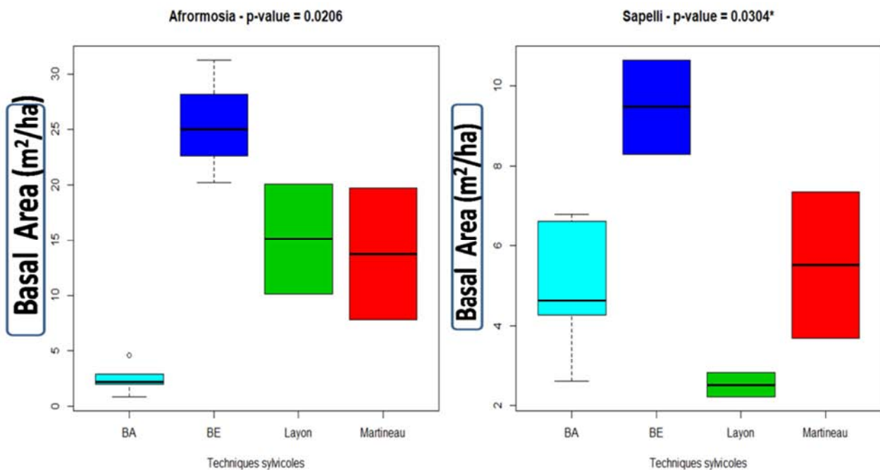
Figure 6. Basal area dispersion values for Pericopsis elata and Entandrophragma cylindricum between the plots of ANR method (assisted natural regeneration). BE (Blanc-Etoc), Layon and Martineau. The box represents the interval in which are regrouped 50% of basal area and the thick bar in the box indicates the average basal area. the lower bar indicates the minimum basal area and the upper bar the maximum basal area.
